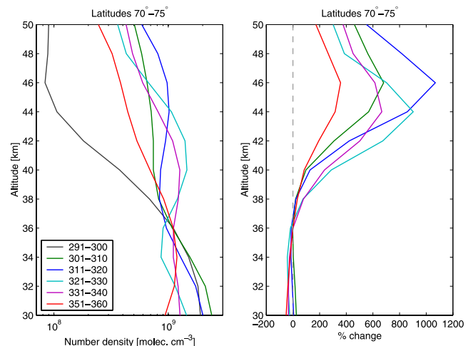
Figure 2. Like Figure 1 but for \text{NO}_2 at altitudes 30–50 km.
