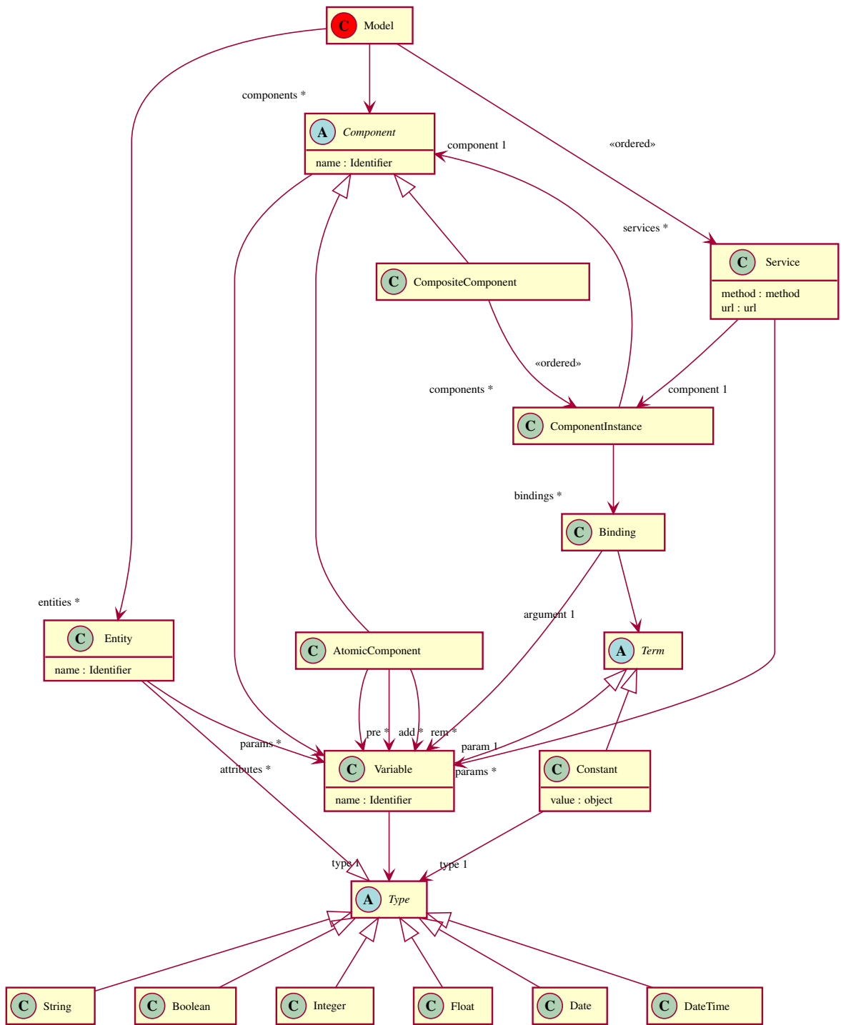
Figure 1: Meta-model diagram
