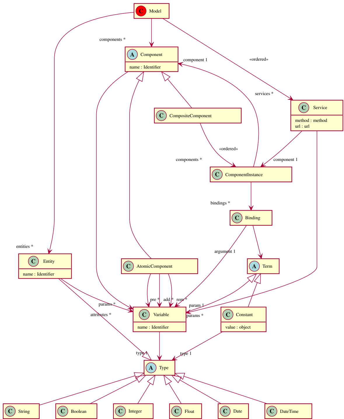
Figure 1: Meta-model diagram
