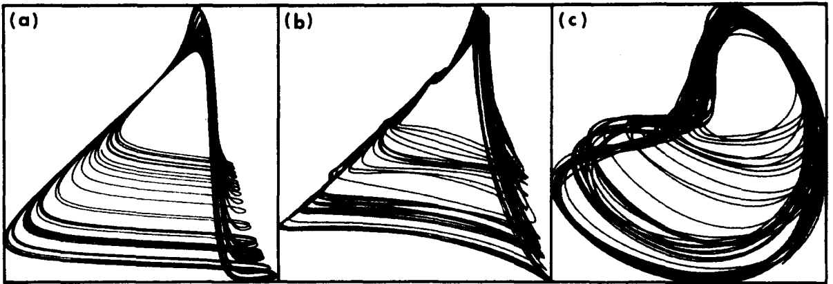
Fig. 8. a) Unfiltered experimental data for the Belousov–Zhabotinskii reaction [2]; b) the same data, low-pass filtered with a filter cutoff of 0.046 Hz, compared to the mean orbital frequency of 0.009 Hz. Our estimate of \lambda_1 for these data was only 5% lower than the estimate from the unfiltered data. Replacement frequencies in the region of stationarity for these results were approximately 0.005 Hz. c) the data are over-filtered at 0.023 Hz. \lambda_1 differs by only 20% from the exponent estimate for unfiltered data.
