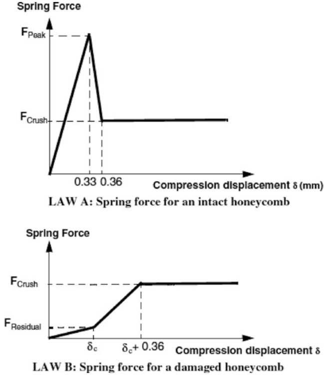
Fig. 60 Spring forces
