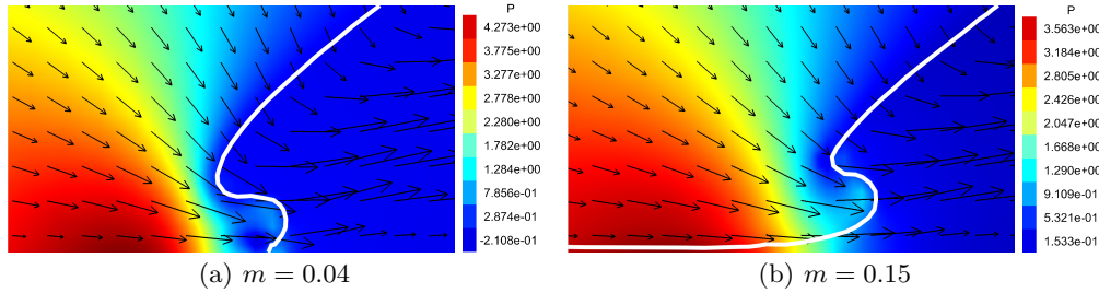
FIGURE 10. Pressure (color) and velocity (arrows) fields at time t = 0.04 for the two different splashing mechanisms at \alpha = 0.003 . On the left the detachment splash for m = 0.04 and on the right the jet splash for m = 0.15 . In the latter case the liquid layer is skating on a thin gas film, and the velocity field in the liquid is almost parallel, while on the left, the liquid is arrested by the substrate, leading to a weaker and more complex velocity field, and higher pressure.
