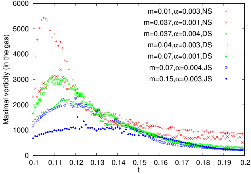
FIGURE 14. Evolution of maximal vorticity in the gas as a function of time for different viscosity ratios ranging from m = 0.01 to m = 0.15 and \alpha = 0.001 to \alpha = 0.004 , covering the different splash and spreading regimes. NS represents non-splashing spreading, DS represents the detachment-splash regime and JS the jet-splash behavior.
