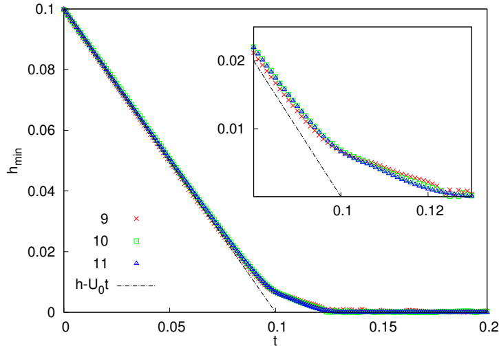
FIGURE 4. Evolution with time of h_{\min}(t) , the minimal air thickness in the numerics, for different maximum refinement levels n (numbers indicated bottom left of the figure) for m = 0.1 and \alpha = 0.001 . The grid size is then proportional to 1/2^n near the substrate. Although small deviations can be observed between the different levels, we observe a rapid convergence of the results. The straight line indicates the free fall of the drop and the inset shows a zoom of the figure near the time where the bubble is entrapped.
