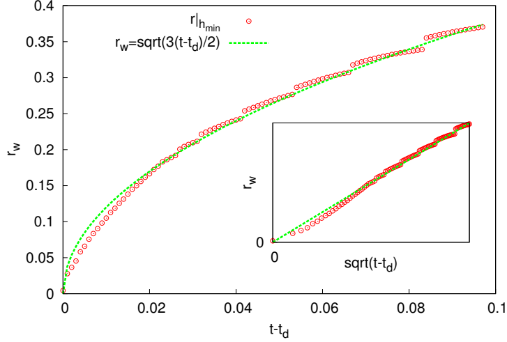
FIGURE 5. Radius r_w , defined as the radius of minimal height as a function of time t - t_d , where t_d = 0.102 is the time at which the dimple beneath the drop appears, for \alpha = 0.001 and m = 0.1 . The inset shows the relation between r_w and \sqrt{t - t_d} . Symbols denote the temporal evolution of the r -coordinate of the h_{min} -point and the dashed curve represents the law r_w = \sqrt{3(t - t_d)/2} .
