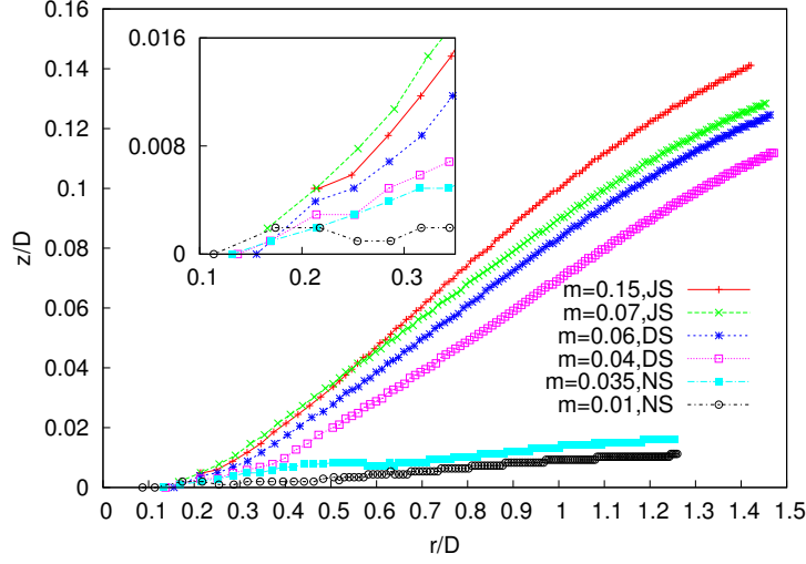
FIGURE 11. Evolution in time of the position of the rim of the liquid sheet for various viscosity ratios m = 0.01, 0.035, 0.04, 0.06, 0.07, 0.15 (as indicated on the right table in the figure) with a constant density ratio \alpha = 0.003 . NS represents non-splashing spreading, DS represents the detachment-splash regime and JS the jet-splash behavior. Inset shows a zoom at small times (around r/D \sim 0.3 ). The position of the rim is defined as the maximum r -coordinate of the expanding liquid lamella. The local minimum observed around r/D \sim 0.6 for m = 0.035 corresponds to the formation of a liquid rim on the spreading lamella.
