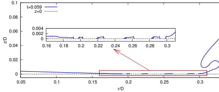
FIGURE 6. The expanding lamella after bubble entrapment ( t = 0.059 ) for the same parameters as in figure 5. The liquid-gas interface is drawn while the solid surface is the dashed line plotted at z = 0 . Small bubbles are entrapped within the wetted area due to the rapid expansion of the lamella, as displayed in the inset that shows a zoom of the wetted area.
