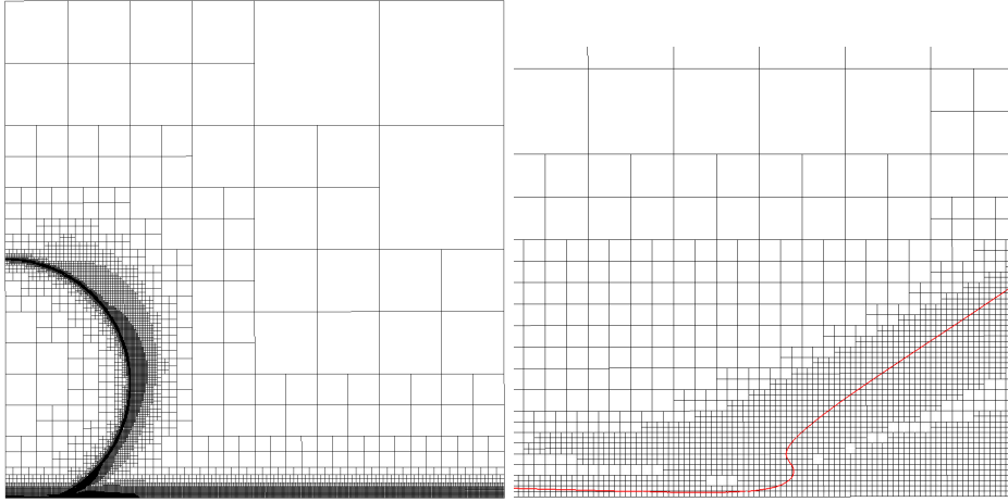
FIGURE 3. Snapshots of the adaptive mesh refinement at two different instants of the impact: left, just before impact where most of the refinement is concentrated on the interface and solid surface. On the right figure, a zoom after the impact when a layer of liquid is skating above the solid surface, the red curve representing the interface.
