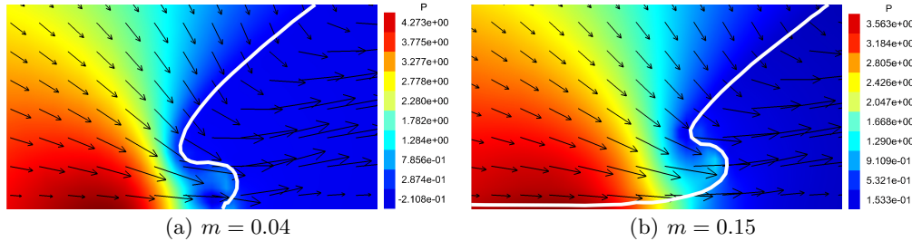
FIGURE 10. Pressure (color) and velocity (arrows) fields at time t = 0.04 for the two different splashing mechanisms at \alpha = 0.003 . On the left the detachment splash for m = 0.04 and on the right the jet splash for m = 0.15 . In the latter case the liquid layer is skating on a thin gas film, and the velocity field in the liquid is almost parallel, while on the left, the liquid is arrested by the substrate, leading to a weaker and more complex velocity field, and higher pressure.
