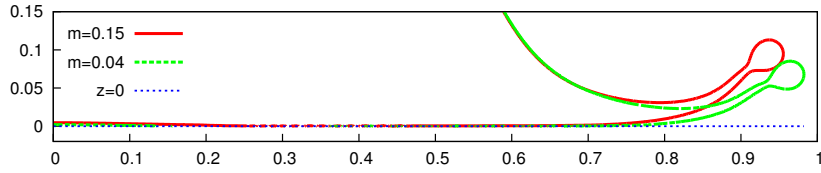
FIGURE 9. Interface profiles at the same time t = 0.5 for density ratio \alpha = 0.003 and for the two viscosity ratios m = 0.15 and m = 0.04 at which splash was observed in figure 8. The line z = 0 represents the solid substrate.
