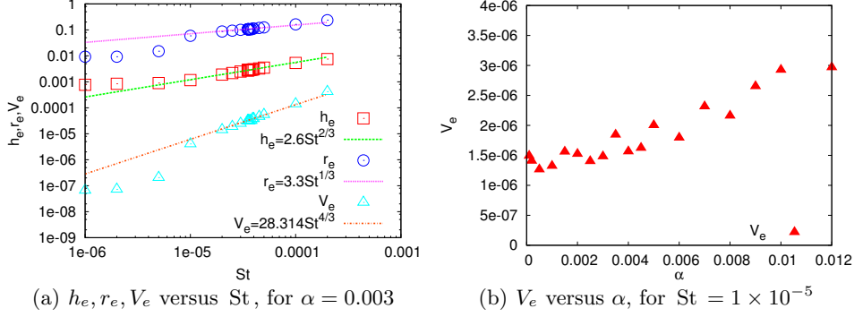
FIGURE 7. (a) Thickness of the gas layer h_e , radius of the first contact point r_e and volume of the central entrapped bubble V_e versus the Stokes number St (logarithmic scale) for density ratio \alpha = 0.003 (this implies m = Re \cdot St = 1000 St ), Symbols represent simulation results. Dashed lines represent the scaling laws h_e = 2.6St^{2/3} , r_e = 3.3St^{1/3} and V_e = 28.314St^{4/3} respectively. (b) V_e versus density ratio \alpha for St = 10^{-5} .
