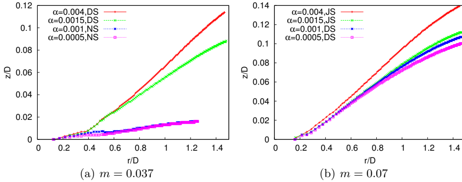
FIGURE 12. Position evolution of the rim of the thin liquid sheet on varying the density ratio \alpha = 0.0005, 0.001, 0.0015, 0.004 with a constant viscosity ratio: (a) m = 0.037 and (b) m = 0.07 . The value of \alpha for each curve is indicated on the top left of each figure. NS represents non-splashing spreading, DS represents the detachment-splash regime and JS the jet-splash behavior. The local minimum observed in (a) around r/D \sim 0.6 for \alpha = 0.001 corresponds to the formation of a liquid rim on the spreading lamella.
