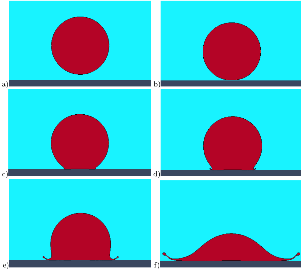
FIGURE 1. Snapshots of droplet impact on a solid substrate obtained by solving the axisymmetric two-phase Navier-Stokes equations using the Gerris solver, for Re = 1000 , We = 370 , \alpha = 0.003 and m = 0.15 . The images correspond to the dimensionless times a) t = -0.1 , b) t = 0 , c) t = 0.048 , d) t = 0.087 , e) t = 0.2 and f) t = 0.6 .
