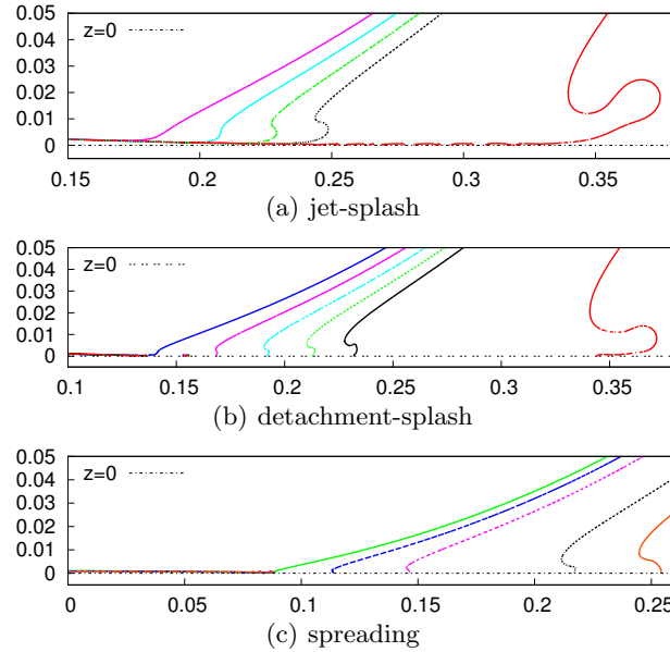
FIGURE 8. Interface evolution in time at the early stage of impact for \alpha = 0.003 but different viscosity ratios m : (a) jet-splash, m = 0.15 , the interfaces from left to right correspond to t = 0.025, 0.030, 0.035, 0.040, 0.080 respectively; (b) detachment-splash, m = 0.04 , the interfaces from left to right correspond to t = 0.015, 0.020, 0.025, 0.030, 0.035, 0.080 respectively; (c) spreading, m = 0.01 , the interfaces from left to right correspond to t = 0.007, 0.010, 0.015, 0.030, 0.040 respectively. The line z = 0 represents the solid substrate.
