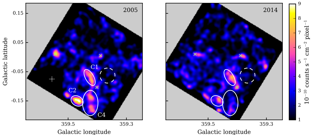
Fig. 1. Chandra continuum-subtracted images of the Fe K\alpha emission in Sgr C for the observations taken in 2005 ( left ) and 2014 ( right ). The maps are in units of counts s^{-1} \text{cm}^{-2} \text{pixel}^{-1} with a pixel size of about 1'' , and smoothed using a Gaussian kernel of 20-pixel radius. The regions of interest (Sgr C1, Sgr C2, and Sgr C4) are marked by the solid ellipses (see Table 2). The dashed circle shows the control region. The white cross marks the position of the X-ray transient KS 1741–293, which has been removed from the 2005 dataset. The green crosses mark the positions of bright point sources ( F_{0.5-8 \text{ keV}} > 10^{-5} \text{ counts s}^{-1} \text{cm}^{-2} ) from the catalogue of Muno et al. (2006) that remain visible in the 6.4 keV band after continuum subtraction.
