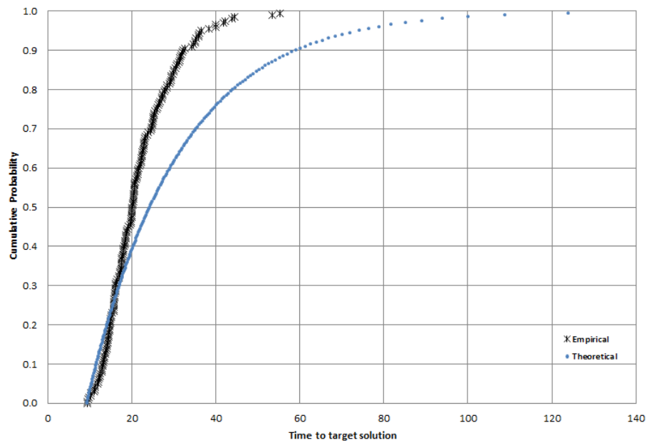
Figure 5: TTT plots produced for instance y.4.20.4 - target value equal to 19.
