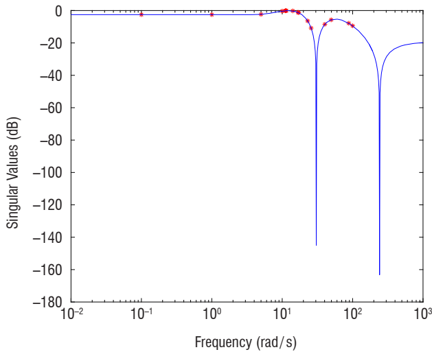
Figure 4 – Singular values
