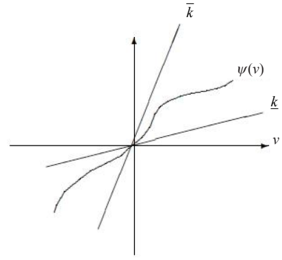
Figure 2 – Sector non-linearity
