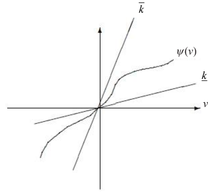
Figure 2 – Sector non-linearity
