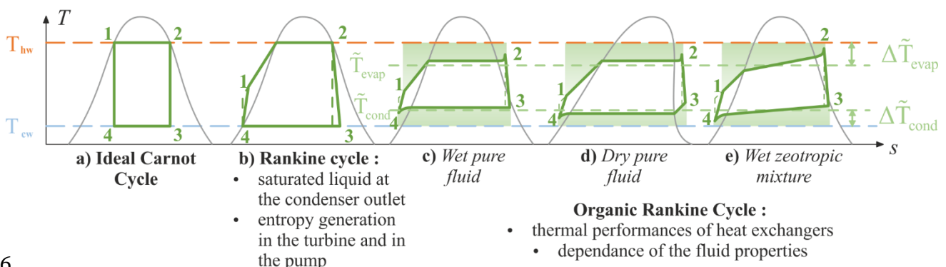
16 17 Figure 2. T-s diagram of thermodynamic cycles progressing from ideal to real
