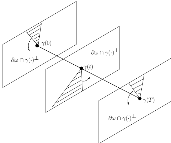
Figure 2: Locally around \gamma(t) , \partial\omega \cap \gamma(t)^\perp is the complement of the hatched area.
