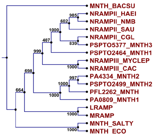
Figure 2 Phylogenetic tree for Nramp family of manganese transporters using neighbour joining method with 1000 bootstrap replicates. It depicts the grouping of various orthologs of Pseudomonas species within this family. BACSU, Bacillus subtilis ; HAEI, Haemophilus influenzae ; SAU, Staphylococcus aureus ; CGL, Corynebacterium glutamicum ; MYCLEP, Mycobacterium leprae ; CAC, Corynebacterium acetylicum ; SALTY, Salmonella typhimurium ; ECO, Escherichia coli .
