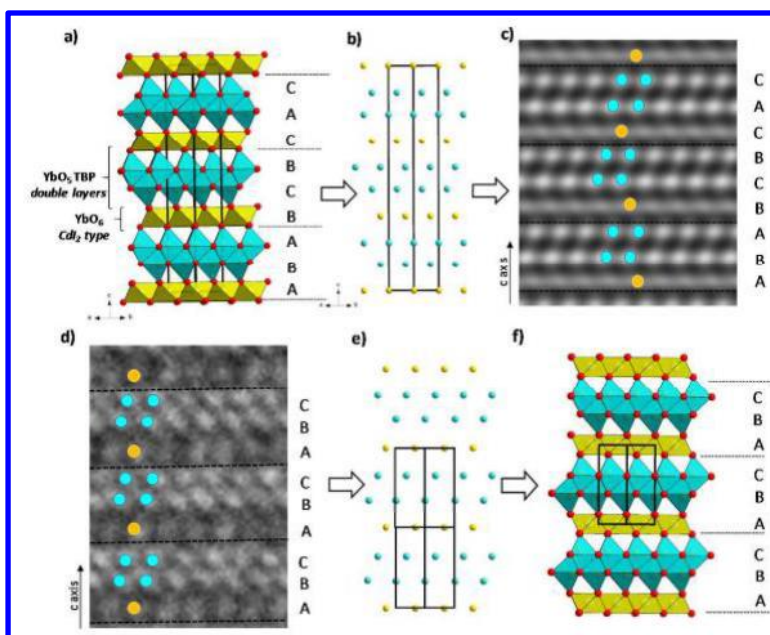
Figure 1: Structure of \text{YbFe}_2\text{O}_4 and deduction of the average \text{YbFe}_2\text{O}_{4.5} crystal structure: a,b ) The crystal structure of \text{YbFe}_2\text{O}_4 and its cationic packing. c) Matching with the [010] simulated HREM image for defocus and thickness values \Delta f = 0 \text{ \AA} , \Delta t = 24.2 \text{ \AA} . d) \text{YbFe}_2\text{O}_{4.5} : the [010] experimental HREM image. e,f) Deduced cationic packing and structural model.
