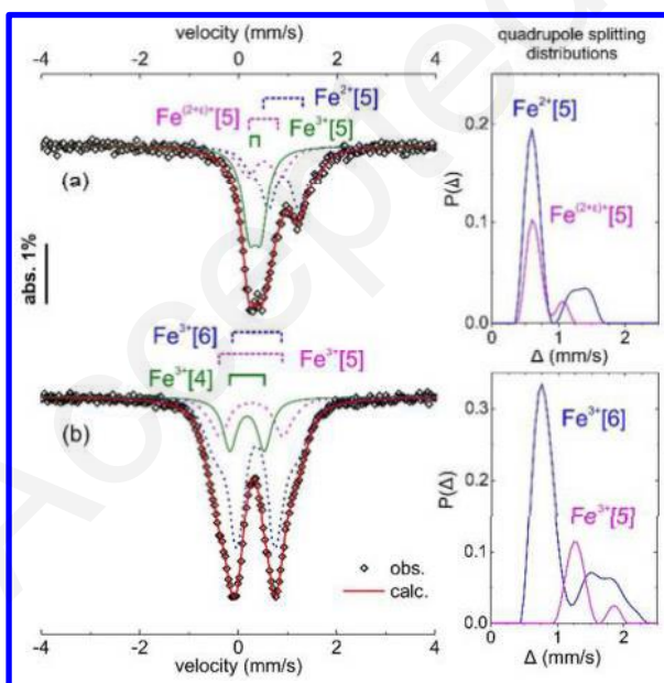
Figure 3: Room temperature ^{57}\text{Fe} Mössbauer spectrum of a) \text{YbFe}_2\text{O}_4 and b) \text{YbFe}_2\text{O}_{4.5} . The components with dashed lines were calculated considering a distribution of the quadrupole splitting parameter.
