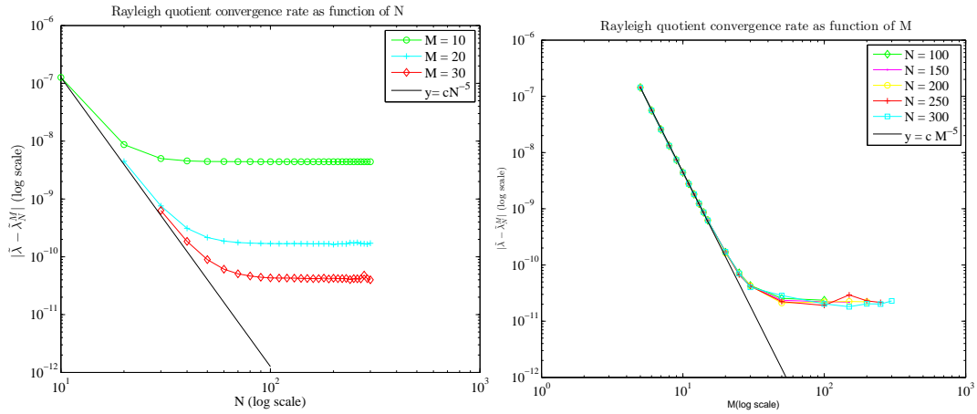
FIG. 4. Numerical errors |\tilde{\lambda} - \tilde{\lambda}_N^M| (Fourier approximation), as functions of N (left) and M (right) (in log-log scale).
