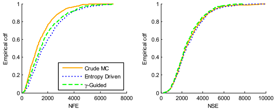
Fig. 11. Empirical cdfs of the NFE (left) and of the NSE (right) for crude MC (light line), for an entropy-driven method (dark dotted line), and for the preliminary guided exploration with \gamma = 1 (light dashed line) with flow rate parameters [\phi_a, \phi_b, \phi_c] = [8, 2.2, 6] \cdot 10^4 \text{m}^3/\text{day} .
