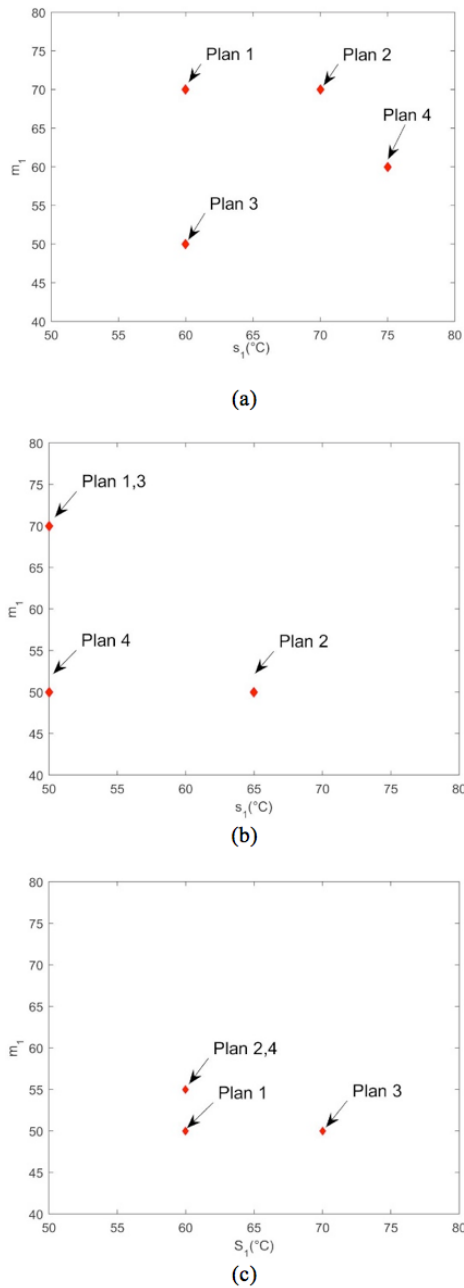
FIGURE 3. Optimal results of different prior distributions under the objectives of (a) relative entropy, (b) quadratic loss function and (c) D-optimality.
