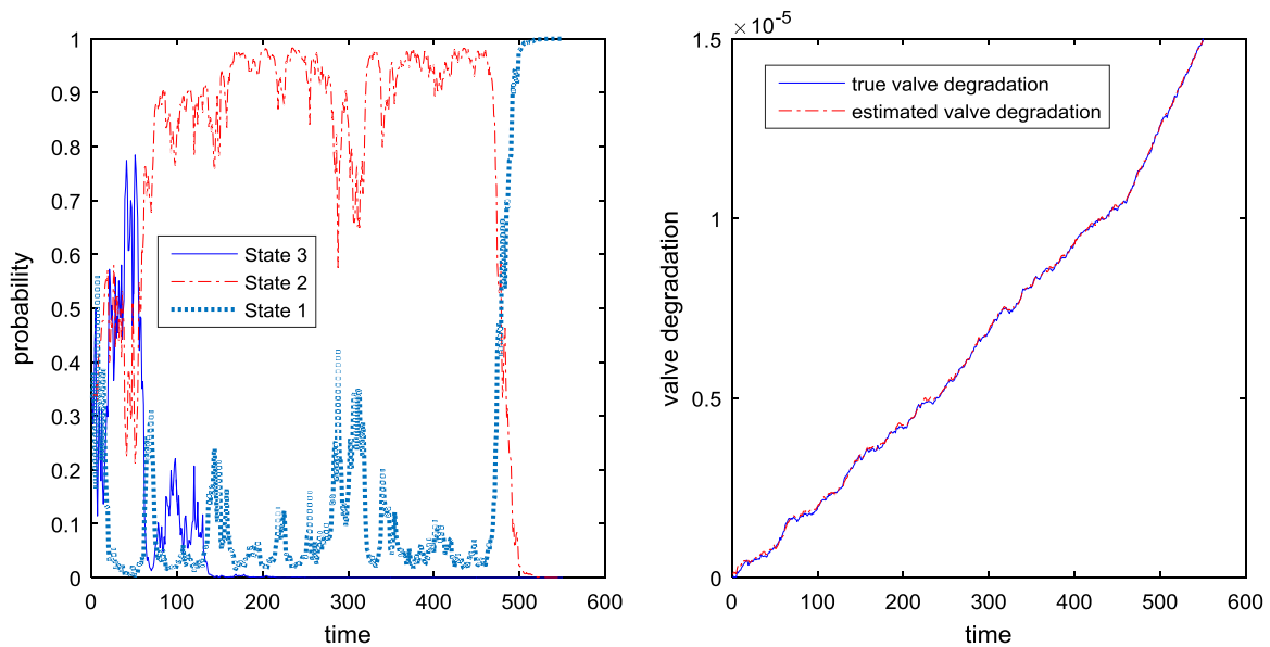
Fig. 5. True and estimated pump (left) and valve (right) degradation state of scenario 1.
