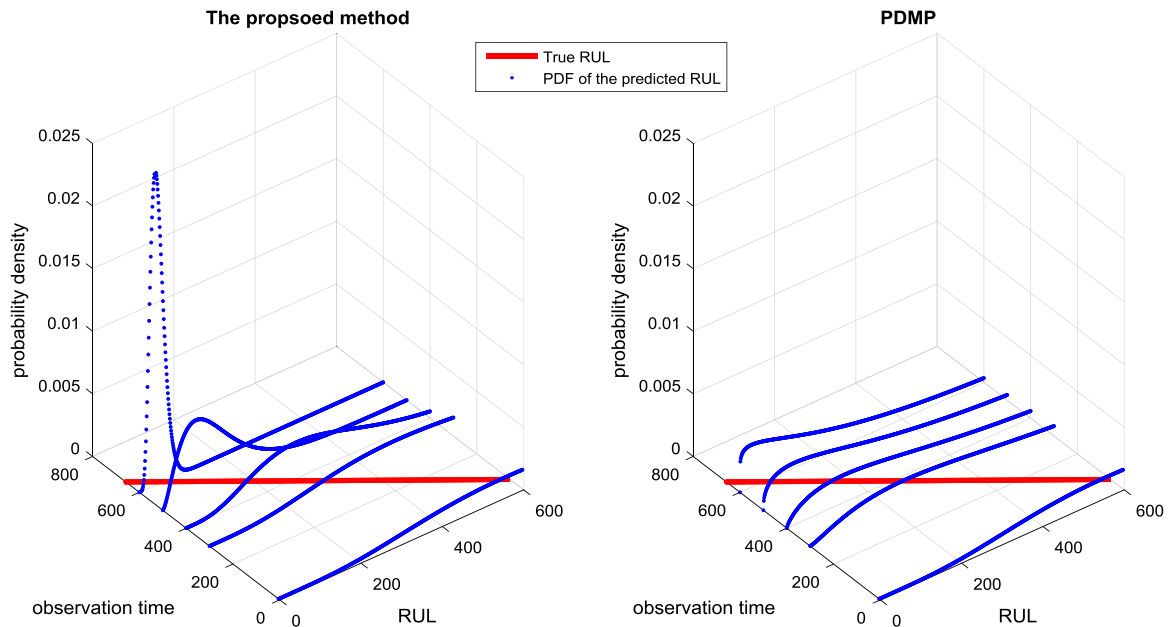
Fig. 24. PDFs of the predicted RUL for test scenario 2, given the true system state at time 0 and the monitored data until different times, using the proposed method and PDMP.
