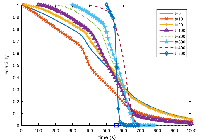
Fig. 9. Reliability of the monitored system, given the data monitored until different observation times for Scenario 1. (The true failure time is marked as a square on x axis.).
