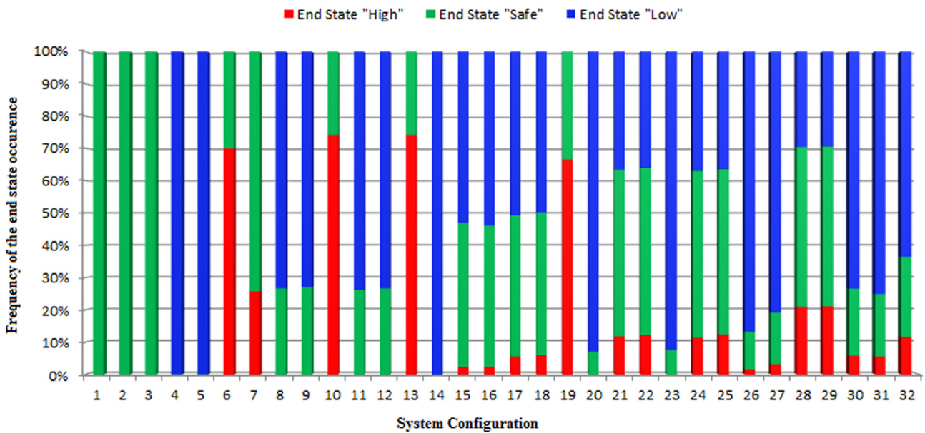
Fig. 4. Histograms of the frequency of end states for each of the 32 system configurations listed in Table 3.
