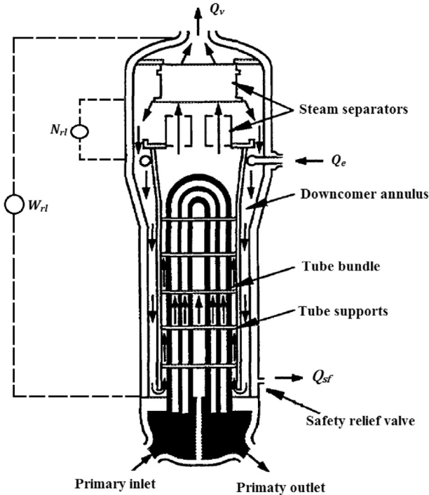
Fig. 5. Schematic of the UTSG (Kothare et al., 2000).
