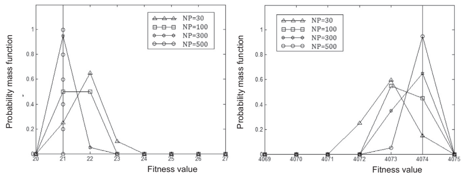
Fig. 10. Pmfs of the \bar{x}_{opt} fitness values obtained with BDE, using the “Penalty” fitness function (left) and the “One complement” fitness function (right).
