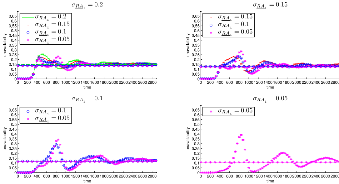
Fig. 11. Sensitivity of Unavailability to \sigma_{RA_1} .
