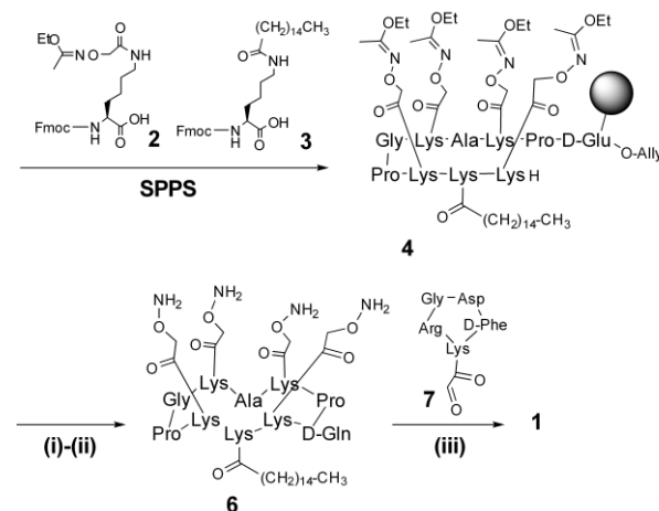
Scheme 1. Synthesis of 1 : (i) 1 equiv. Pd(PPh 3 ) 4 , 100 equiv. PhSiH 3 ; (ii) 2 equiv. PyAOP, DIPEA (pH 8.0); TFA, TIS, H 2 O (90:5:5); (iii) 4.4 equiv. 7 , acetic acid, H 2 O, CH 3 CN (50:25:25).
