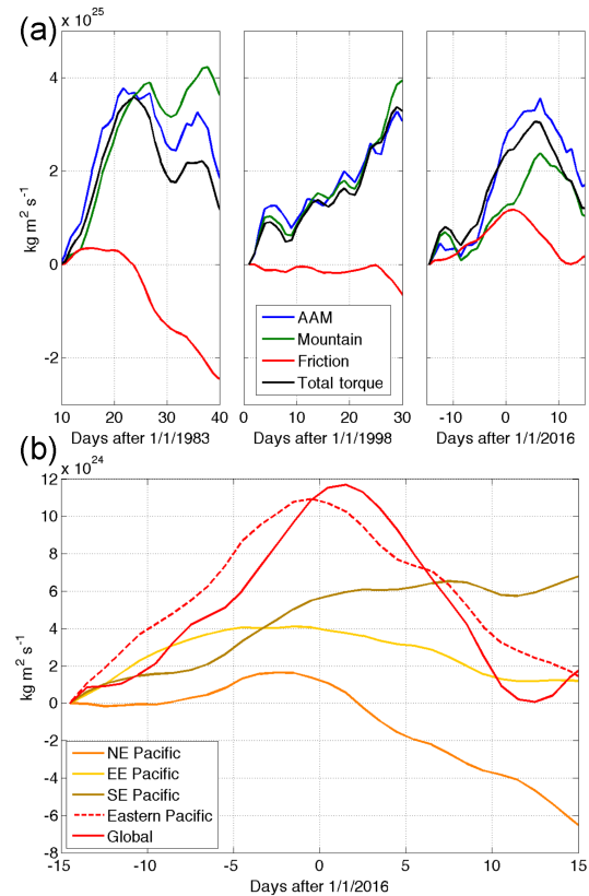
Figure 4. (a) The integrated torques compared to AAM during the three events and (b) the integrated friction torque with contribution from the different regions of the Pacific Ocean during the 2015–2016 event.
