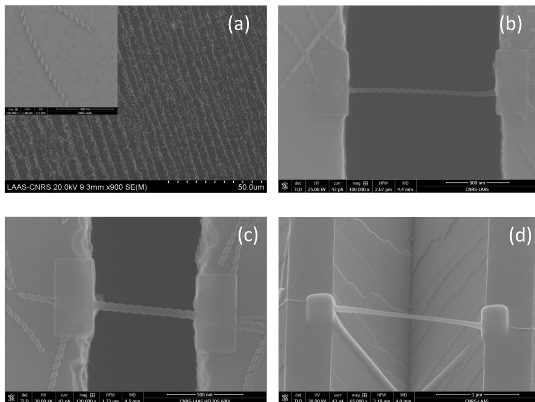
Figure 1. (a) SEM image of silica NS deposited on a silicon substrate using oriented capillary assembly with a closer view on individual ones in the inset. SEM images showing the morphologies of suspended NS after metallization and clamping by FIB. (b) EBID thin coating. (c) EBID thick coating. (d) IBID thick coating.
