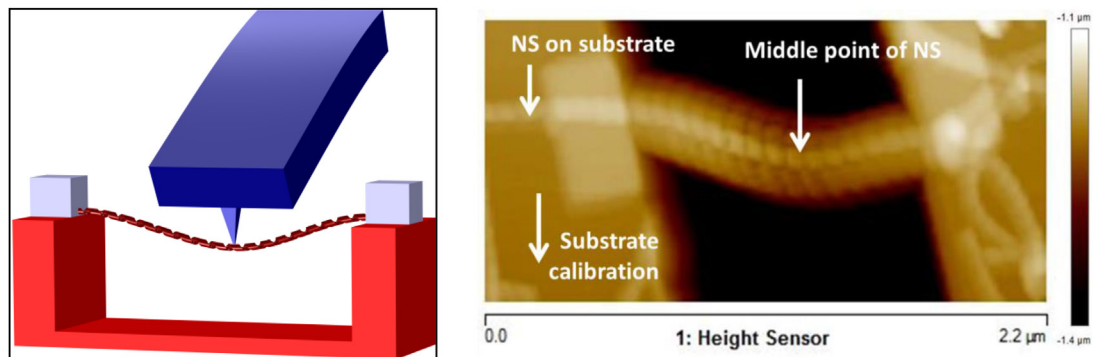
Figure 4. Principle of the 3-point bending test using AFM. Two force–distance ( F – d ) curves are recorded: one on the nanostructure resting on the substrate, and one at the midpoint of the doubly-clamped suspended nanostructure. The slope obtained from the NS on the substrate gives the effective stiffness k_C of the AFM cantilever, while the slope S obtained at the midpoint from the suspended NS corresponds to the contribution of k_C and k_{NS} , the stiffness of the NS. Using this procedure, k_{NS} can be easily determined.
