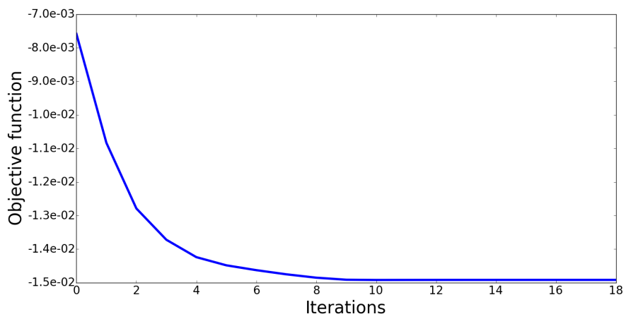
Figure 10: Convergence history for the optimization of the 2D composite sandwich plate.
