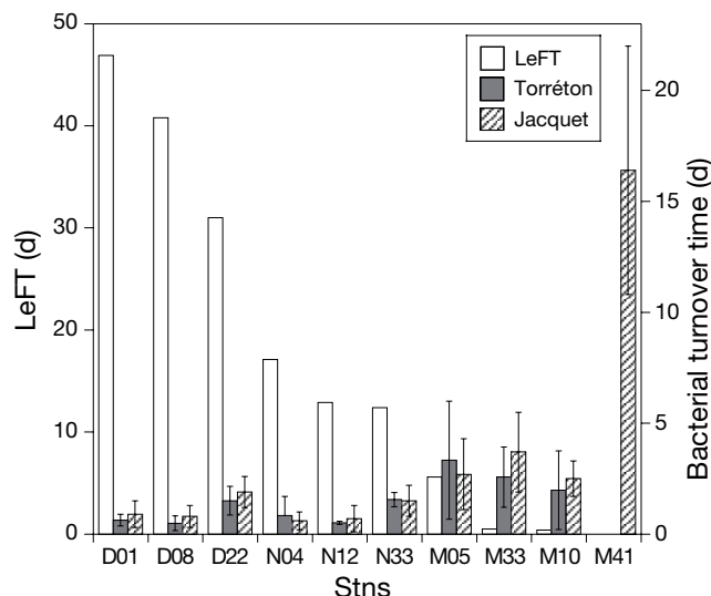
Fig. 5. Local e-flushing time (LeFT) and bacterial turnover times at the sampling stations. Water residence times were calculated for the most common trade wind conditions of 8 \text{ m s}^{-1} (Mari et al. 2007a). Bacterial turnover times were calculated from 2 data sets available from the study stations (Jacquet 2005, Torr ton et al. 2007). The Torr ton data set was obtained from cruises in September 2000, June 2003, and October 2004, and the Jacquet data set was from April–May 2002, August 2002, and January 2003. Bacterial production was calculated from ^3\text{H} -thymidine incorporation rates (TdR) using a conversion factor of 2.85 \times 10^8 \text{ cells mol}^{-1} \text{ TdR} obtained for the environment (Jacquet 2005)
