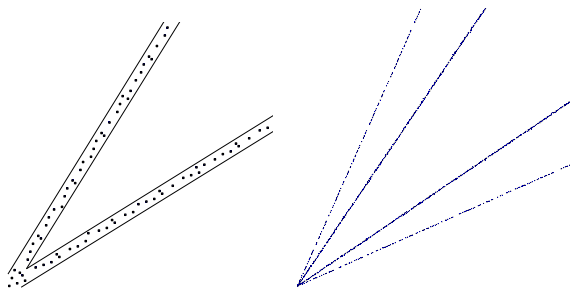
FIGURE 6. Some initial P-positions have been computed for MAHARAJA NIM and (1, 2)-GDWN respectively. The leftmost picture indicates that we are able to capture the behavior of MAHARAJA NIM's upper P-positions within a narrow stripe of slope \phi . On the other hand, we have proved that the P-positions of GDWN to the right will eventually depart from any such stripe, however wide we make it. Extensive computations make us believe that perhaps the upper pair of P-beams' slopes will converge to the accumulation points 1.478... and 2.248... respectively.
