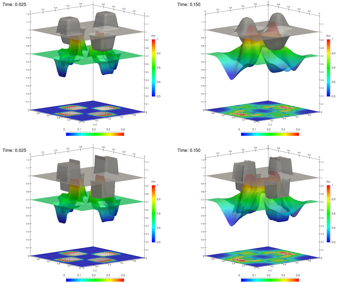
Figure 7: Case 2: the comparison of (\varrho, \mathbf{q}, Z) -method (top) and (\varrho, \mathbf{q}) -method/SL (bottom) at time 0.025 (left), and 0.150 (right).
