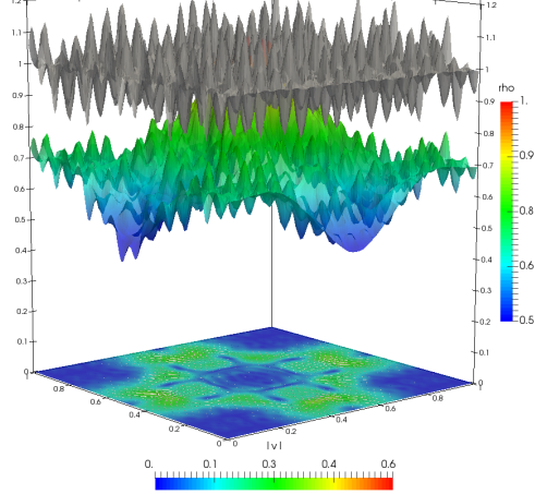
Figure 8: Case 3: the comparison of (\rho, \mathbf{q}, Z) -method (top) and (\rho, \mathbf{q}) -method/SL (bottom) at time 0.025 (left), and 0.150 (right).
