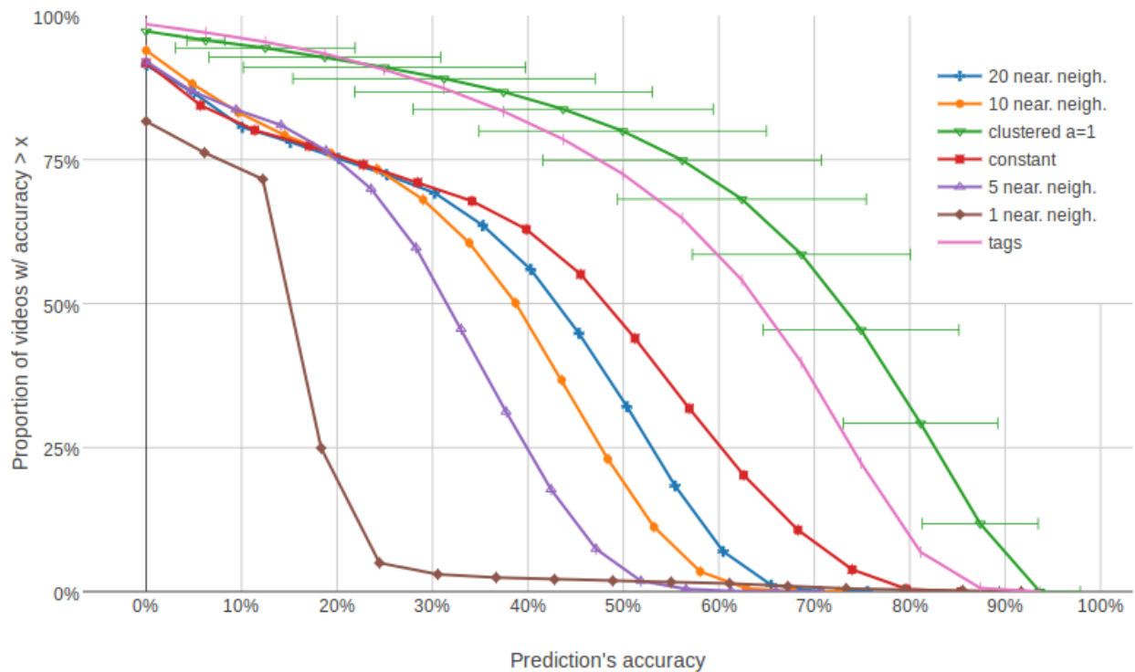
Figure 12: CDF of the accuracy of geographic distribution of videos' views prediction using a different number of nearest neighbours, with the two baselines and the result of clustered prediction with \alpha = 1 .
