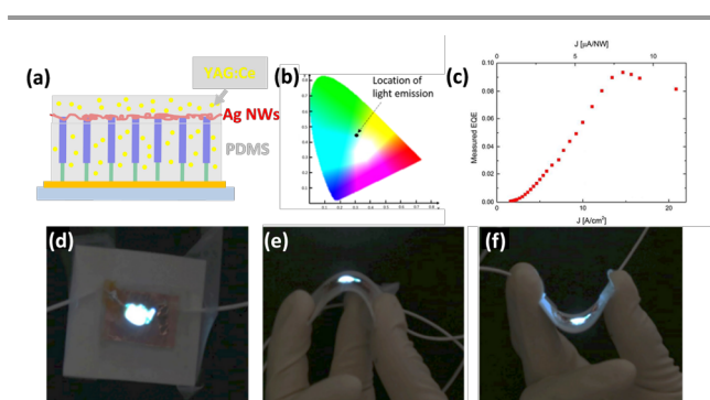
Fig. 8 (a) Schematic of the flexible white LED. (b) CIE 1931 chromaticity diagram of flexible white LEDs under injection current density of 3.9 \text{ A/cm}^2 (chromaticity coordinates x=0.3011 , y=0.4688 ; CCT= 6306 K; CRI=54). (c) Room temperature EQE deduced from the measured optical power versus the injection current density. (d)-(f) Photographs of the operating flexible white LED with bending radii of infinity, 5 mm, and -5 mm, respectively. Adapted with permission from ref. 59.
