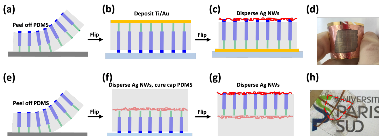
Fig. 3 Schematic of the fabrication process flow of flexible LEDs based on vertical nitride nanowire arrays. Panels (a)–(c) illustrate the fabrication steps for semitransparent LEDs with Ti/Au and Ag nanowires as the back and top contacts, respectively. (d) Photograph of a semitransparent LED. Panels (e)–(g) show the process of fully transparent LEDs with Ag nanowires as both back and top contacts. (h) Photograph of a transparent LED. Adapted with permission from ref. 58.
