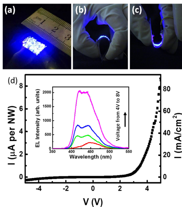
Fig. 5 Mechanical properties of the flexible LED based on vertical nanowire arrays. Photograph of the LED emitting blue light at curvature radii of (a) \infty , (b) 3.5 mm, and (c) -2.5 mm. (d) I-V characteristic of the flexible LED normalized to the number of contacted nanowires (left scale) or to the device surface (right scale). Inset shows the room-temperature EL spectra at various applied biases from 4 V to 8 V. Adapted with permission from ref. 58.
