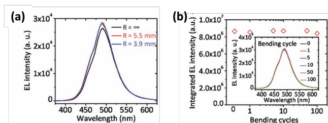
Fig. 6 (a) EL spectra as a function of the bending radius. (b) Integrated emission intensities as a function of bending cycle. Inset shows the EL spectra at different bending cycles. Adapted with permission from ref. 61.
