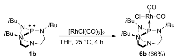
Scheme 1. Synthesis of rhodium complex 6b .
