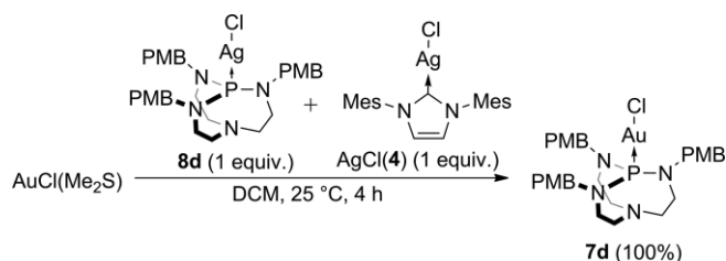
Scheme 4. Competition experiment of transmetalation between a proazaphosphatranane and NHC ligand.
