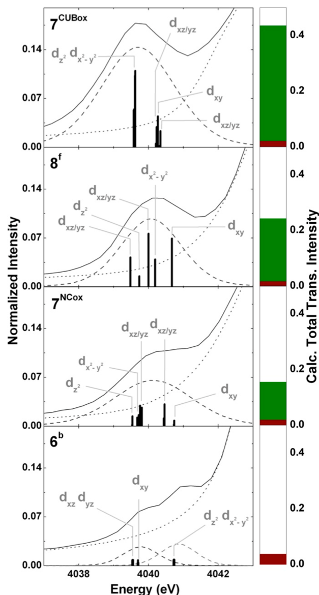
Figure 4. Pre-edges of Ca K-edge with their associated TD-DFT transitions and acceptor orbital assignment. From top to bottom: 7^{\text{CUBox}} , 8^f , 7^{\text{NCox}} , 6^b . (Left) Experimental spectra (black). Spectral fitting: rising edge (dotted lines), pre-edges (dashed lines). Calculated transition intensities (black bars). (Right) Breakdown of contributions to the total calculated transition intensities in terms of total dipole (green) and quadrupole (red) transition intensities, summed over the whole pre-edge. The calculated transition energies were shifted by 50.17 eV, and intensities were multiplied by a factor of 3500.
