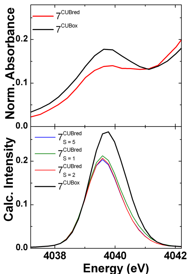
Figure 7. Experimental and calculated Ca K-pre-edge for 7\text{CUBox} and 7\text{CUBred} . Experimental spectra (top). Calculated spectra for 7\text{CUBred} and 7\text{CUBox} (bottom). Calculated pre-edge transitions were approximated as Gaussian–Lorentzian sum peaks (width 1.2 eV, shape 75% Gaussian). A 50.17 eV energy shift was applied, and intensities were multiplied by 3500 units.
