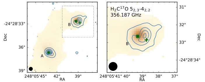
Fig. 1. PILS ALMA continuum map of the IRAS 16293–2422 system at 850 \mu\text{m} . The background image shows the continuum emission, the contours indicate the H 2 C 17 O 5_{2,3}-4_{2,2} line ( E_u = 98.5 K) integrated emission, the star is the position of the continuum peak, and the plus sign the position of the extracted spectrum (one beam, i.e., 0".5, away from the continuum). The continuum image is cut off at 15 mJy ( 3\sigma ) and the line contours start at 25 mJy km s -1 ( 5\sigma ) in steps of 120 mJy km s -1 .
