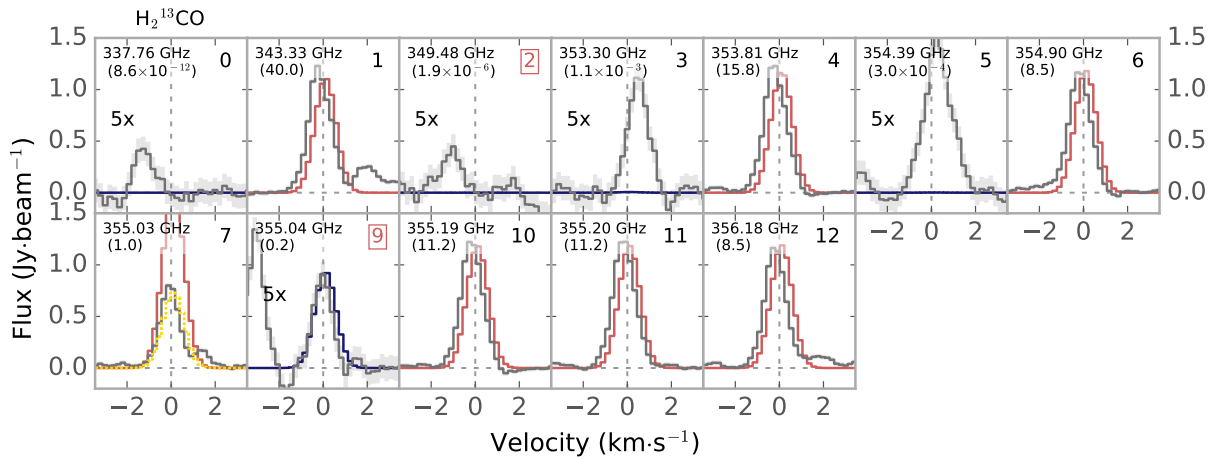
Fig. B.2. All lines of H 2 13 CO with the best fit LTE model overplotted. Synthetic spectra in red indicate optical depth beginning to play a significant role i.e. \tau > 0.6 . Numbers in top right corner with red boxes indicate lines used to fit the column density. The number in parenthesis is the estimated optical depth. The line in panels 9 and 11, at 355.04 and 355.20 GHz could be blended with significantly weaker H 2 C 17 O lines (see panel 5 and 8 in Fig. B.1).
