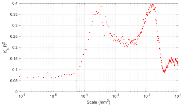
Fig. 11 Multi-scale analysis of the correlation of K_C with SSA
