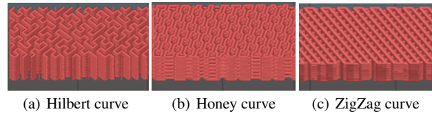
Fig. 15 The 3 different filling strategies
