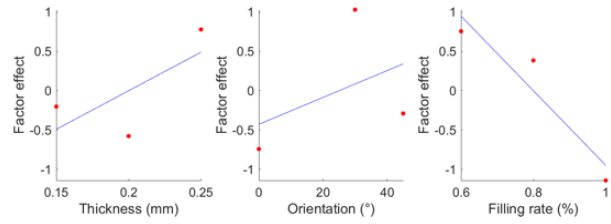
Fig. 14 Factor main effects at the original scale
