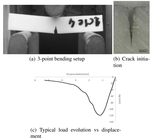
Fig. 10 Description of the cracking tests
