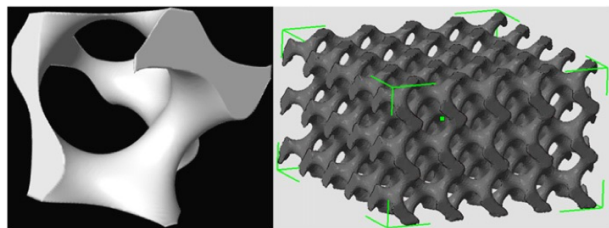
Fig. 1 A unit cell and associated periodic cellular lattice structure [27]
