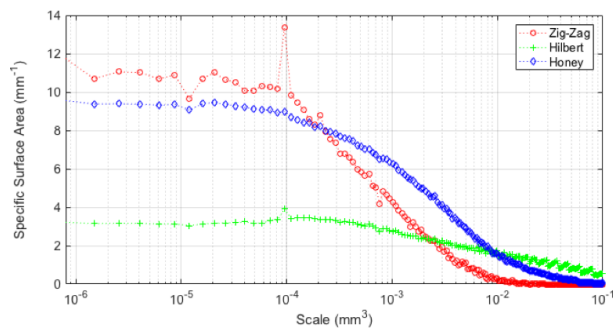
Fig. 16 Pattern geometry comparison using multi-scale analysis
