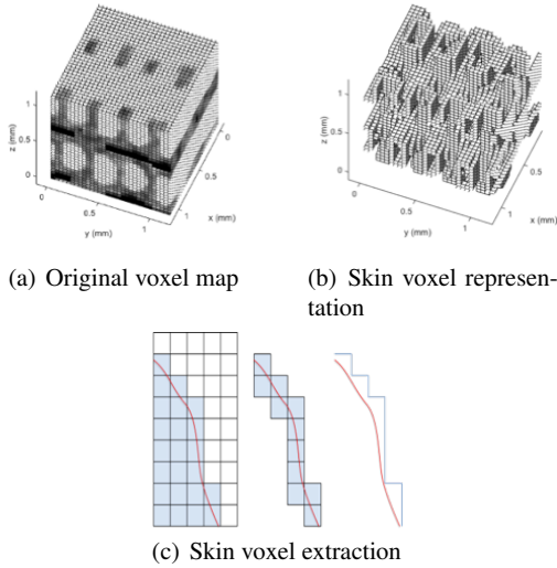
Fig. 7 Voxel representation of surface extraction
