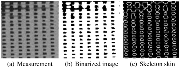
Fig. 6 Surface extraction from the skeleton in a cross-section
