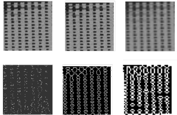
Fig. 9 Surface extraction as a function of scale from left to right (top): Measurement at scale 0.3, scale 1, and scale 3, from left to right (bottom): Surface extraction at scale 0.3, scale 1 and scale 3
