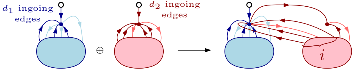
Figure 25: Interpretation of Equation (17) as the combination of two bridgeless maps.
