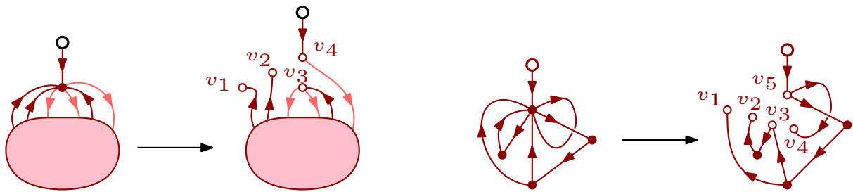
Figure 26: Typical splitting of M_2 , along with an example.
