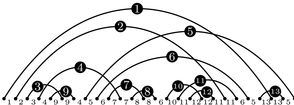
Figure 21: The intersection order version of the diagram of Figure 20.
