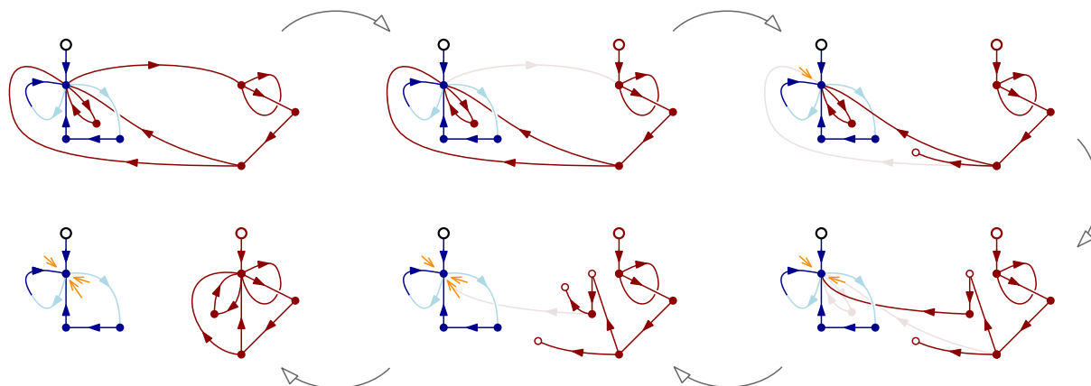
Figure 28: How to recover M_1 and M_2 .
