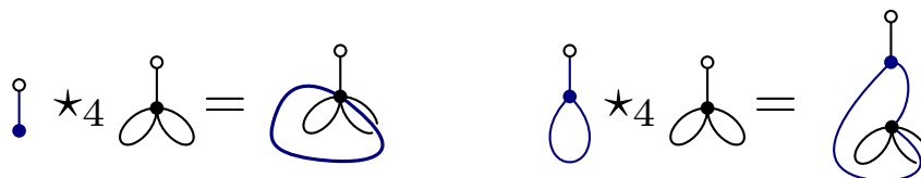
Figure 9: Illustration of the boxed product for bridgeless maps.
