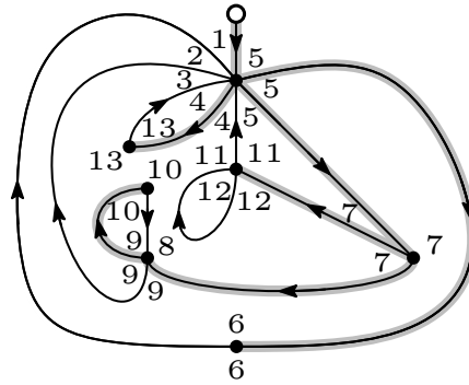
Figure 22: The rightmost DFS of a map and its associated statistics.
