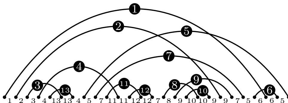
Figure 20: The peeling order of a connected diagram. The covering numbers are also indicated under the intervals.
