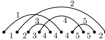
Figure 18: Covering numbers for the intersection order.
