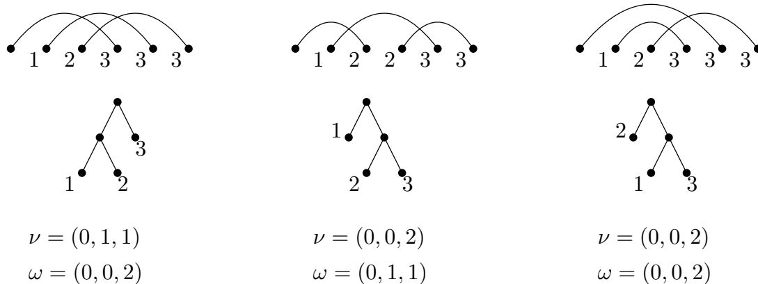
Figure 19: Connected diagrams on 3 chords with only the last chord terminal along with some associated information.
