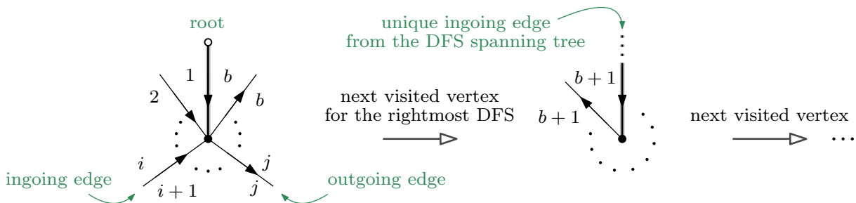
Figure 23: DFS-labeling procedure
