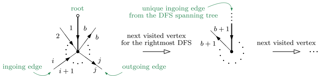
Figure 23: DFS-labeling procedure
