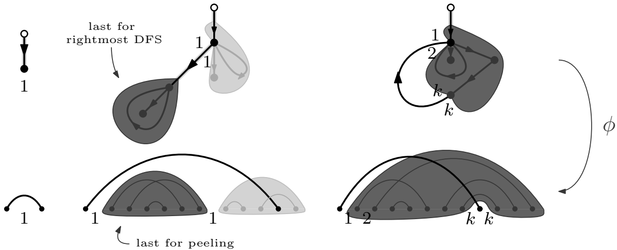
Figure 24: How the statistics evolve from maps to indecomposable diagrams
