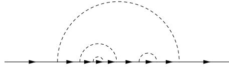
Figure 14: An example of a Feynman graph which occurs in the simpler Dyson-Schwinger equation.
