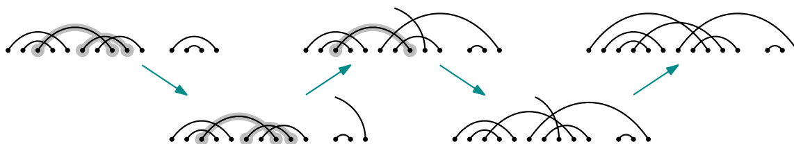
Figure 29: An example of how to combine an indecomposable diagram with another indecomposable diagram in which a subset of top chords is marked. The first diagram has 4 top chords, 2 of which are marked. The second diagram has only one top chord. The combination of both induces 3 top chords, as expected.
