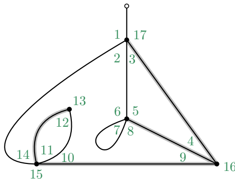
Figure 6: The Bridge First Labeling of a map. The overlined edges correspond to the edges which become bridges during the algorithm described in Subsection 3.2. Alternatively, they form the spanning tree associated to the rightmost DFS.
