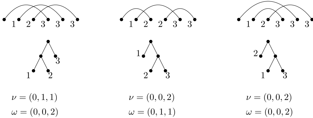
Figure 19: Connected diagrams on 3 chords with only the last chord terminal along with some associated information.
