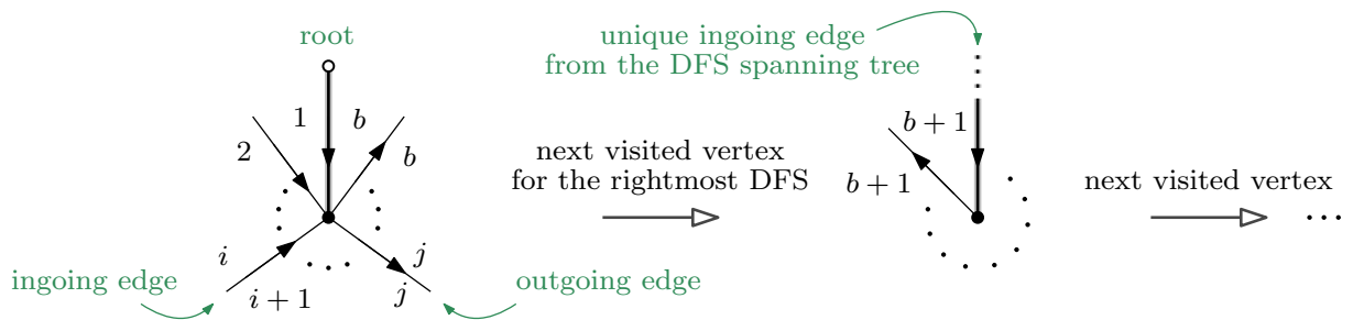
Figure 23: DFS-labeling procedure
