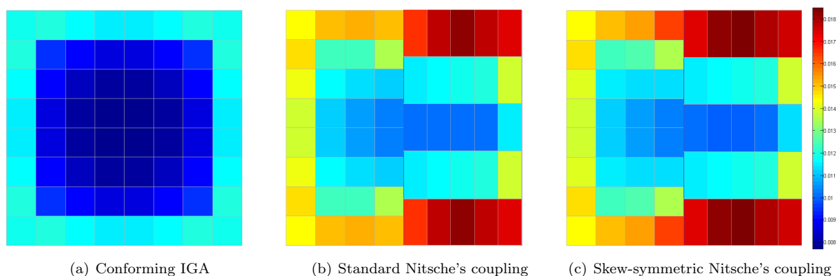
Figure 13: Patch coupling of two plates: element-wise relative errors of displacement field in L^2 norm \|\mathbf{u}^h - \mathbf{u}^{\text{ref}}\|_{L^2(\Omega^e)} / \|\mathbf{u}^{\text{ref}}\|_{L^2(\Omega^e)} . For conforming IGA the mesh is 8 \times 8 , for two patch coupling the meshes are 4 \times 8 and 5 \times 5 .
