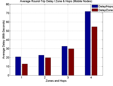
Fig. 10. Average Round Trip Time Delay per zone for Mobile nodes.
