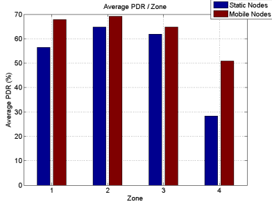
Fig. 8. Average Packet Delivery Rate per zone for Mobile and Tactical static nodes.
