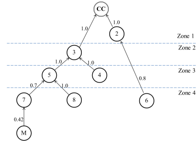
Fig. 6. Snapshot of the network topology after 24 minutes and 13 seconds of the experimentation.
