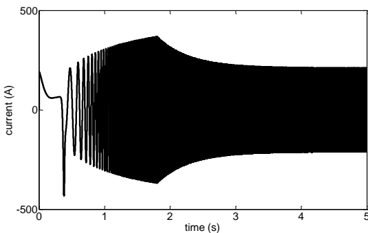
Fig. 2. Stator current
