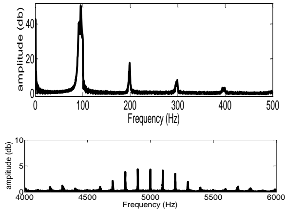
Fig.17. FFT of the current in low and high frequency
