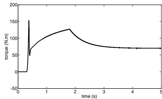
Fig. 4. Machine couples
