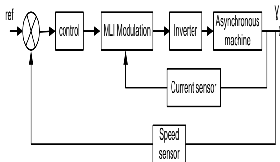
Fig.1. Schematic diagram of the system under study
