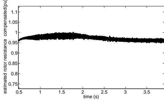
Fig.7. Estimated rotor resistance by the Kalman filter with compensation
