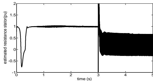
Fig.13 .Estimation rotor resistance for an asymmetrical fault with the stator
