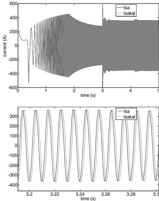
Fig.12. Phase current (Isa), Observed current (Isakal)
