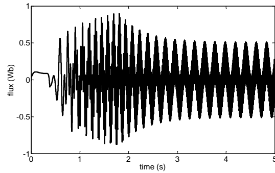
Fig. 3. Stator flux
