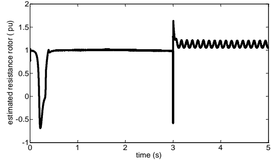
Fig. 9 Estimation resistance rotor for an asymmetrical fault witch the rotor
