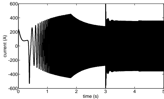
Fig. 10. Stator current of the machine at fault to the stator
