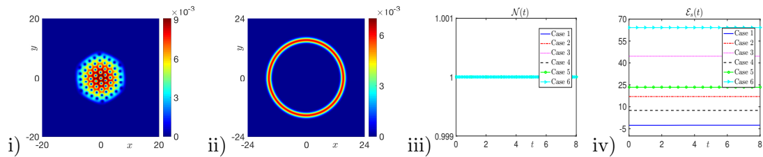
Figure 3. Initial data of Type 1 (i) and Type 2 (ii) and the evolution of the energy and mass for Cases 1 to 6 in Example 3.2.
