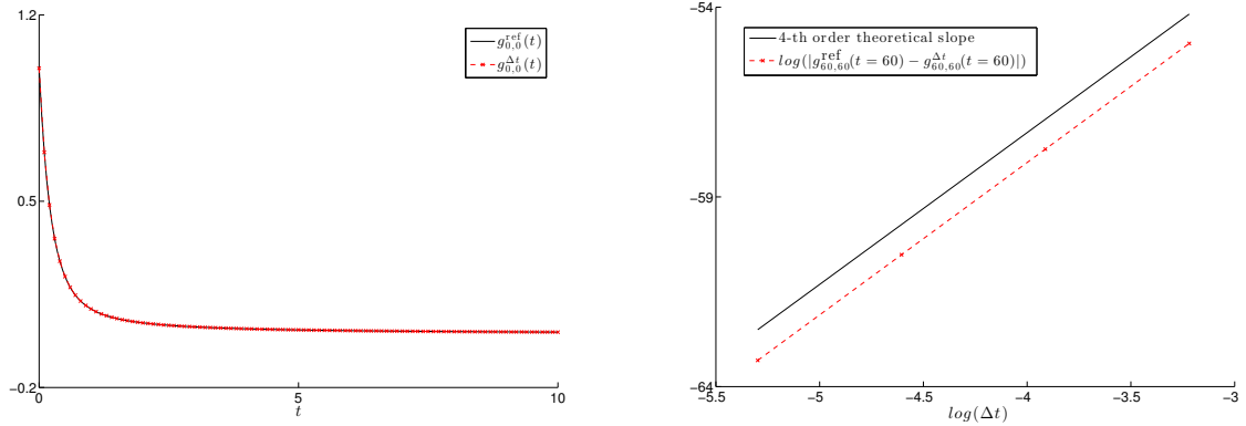
Figure 4: Left: numerical and reference solutions of g_{0,0}(t) for the semi-discretized heat equation. Right: Theoretical and numerical slopes of the convergence rates for the approximation of g_{60,60}(60) .
