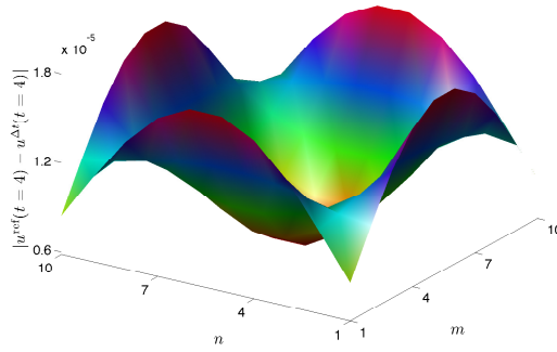
Figure 8: Absolute error |u_{m,n}^{\text{ref}}(4) - u_{m,n}^{\Delta t}(4)| (with \Delta t = 2 \times 10^{-2} ) for the heat equation on the 10 \times 10 square computational domain.
