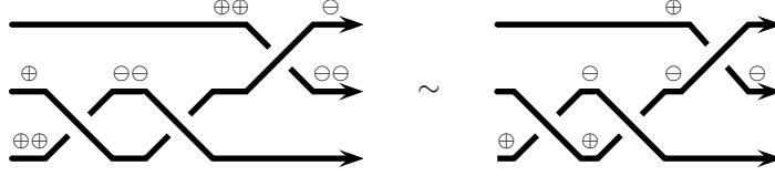
FIGURE 7. Typical charged braid diagrams, represented with \oplus on the i th strand for \rho_i , and \ominus for \rho_i^{-1} : here the diagrams encoded by \rho_1^2 \rho_2 \sigma_1 \rho_2^{-2} \sigma_1 \rho_3^2 \sigma_2^{-1} \rho_3^{-1} \rho_2^{-2} , corresponding to evaluating (\rho_1^2 \triangleright \rho_1) \triangleright 1 with the operation of Prop. 5.3, and the equivalent diagram \rho_1 \sigma_1 \rho_1 \rho_2^{-1} \sigma_1 \rho_3 \rho_2^{-1} \sigma_2^{-1} \rho_2^{-1} , in which two initial \oplus charges have been moved rightwards through \sigma_1 , one cancelling one of the \ominus , and, similarly, two final \ominus charges have been moved leftwards through \sigma_2^{-1} , one cancelling one of the \oplus .
