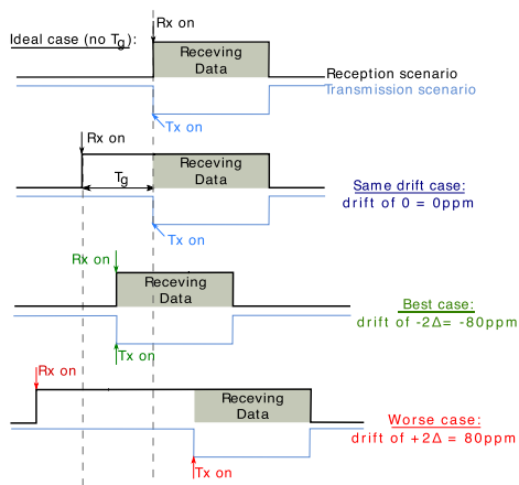
FIGURE 20. Timing relationships.
