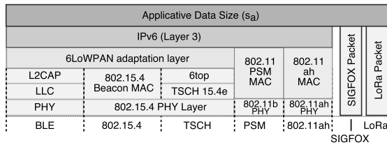
FIGURE 1. Protocol stack of the considered technologies.
