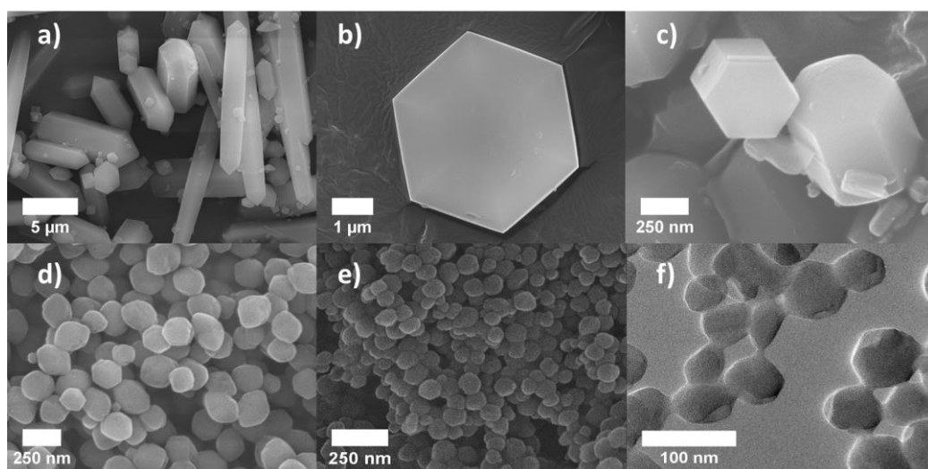
Figure 1. SEM images of the different MIL-96(Al) particles: a) Hexagonal rods (HR), b) hexagonal platelets (HP); c) nanoparticles from reflux in water (NP1); d) nanoparticles from reflux in \text{H}_2\text{O}/\text{DMF} (NP2); e) SEM image of NP3 and f) TEM-bright field image of NP3.
