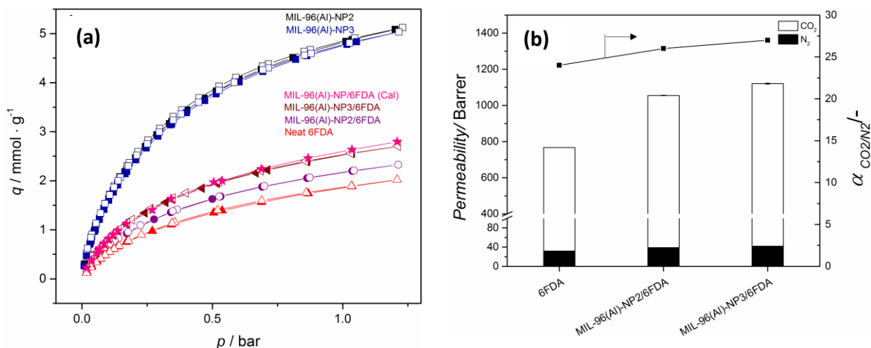
Figure 9. (a) CO 2 adsorption isotherms at 273 K of MIL-96(Al)-NP2 and -NP3, neat 6FDA-DAM, experimental and calculated isotherms of MMMs with 25 wt %. MIL-96(Al)-NP2 and -NP3 loading; (b) Permeation properties for a CO 2 and N 2 mixture (15/85) of MMMs comprising 25 wt.% of MIL-96(Al)-NP2 and -NP3 as filler and 6FDA-DAM as polymer matrix at 298 K and 2 bars feed pressure. Permeate side atmospheric with helium as sweep gas.
