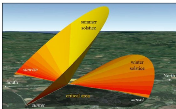
Figure 12: 3D envelop of the reflected rays embedded into Google Earth; applicable to fix structures only.
