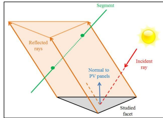
Figure 9: Intersection between a segment and the infinite triangular prism derived from the reflection of the incident sun ray on the PV panels located in the triangular facet.
