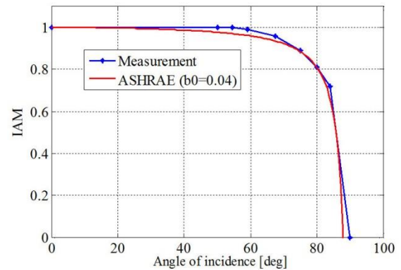
Figure 7: IAM profile of glass-protected PV panels based on ASHRAE modelling ( b_0=0.04 ) and measurements of a specific PV panel performed by Sandia National Laboratories.
