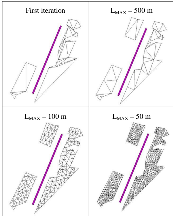
Figure 5: Meshing of the PV plant using two Jordan polygons depending on the maximum side length ( L_{MAX} ) of the triangular facets; runway is highlighted in purple.
