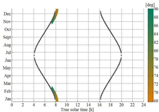
Figure 11: Characterization of the identified impacts through available physical quantities, here the angle between the reflected ray and the user's visual field is analyzed.
