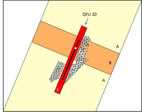
Figure 6: Location of the PV plant within the protection areas (A, B and C) as defined by the French DGAC.
