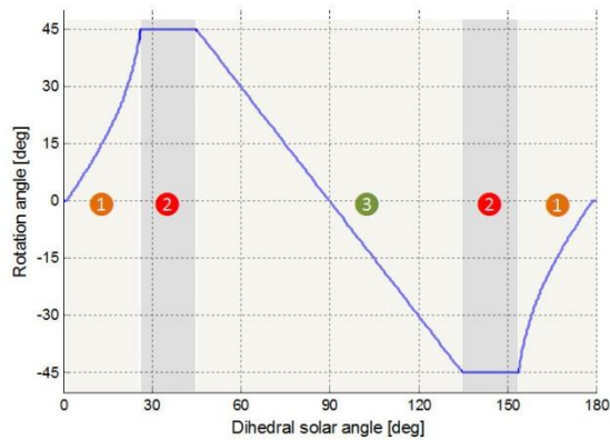
Figure 8: Daily kinematic profile of the 1-axis trackers depending on the dihedral solar angle, highlighting three different modes: backtracking (1), maximum rotation angle (2) and perfect 1-axis tracking (3); applicable whatever the day in the year.
