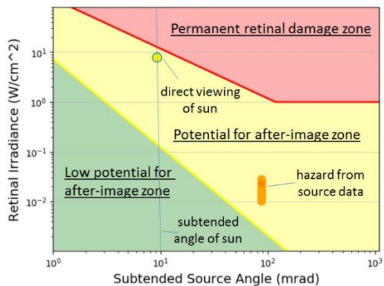
Figure 2: Impact of different retinal irradiances as a function of subtended source angle for short-term exposures.
