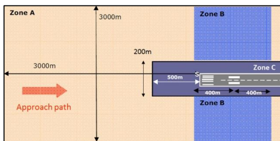
Figure 3: Definition of the three geographical zones A, B and C as per DGAC's requirements depending on the airport threshold (beginning/end of runway) and the touchdown point. The distances are different for a helicopter final approach and take off area (FATO) but the definition remains the same.
