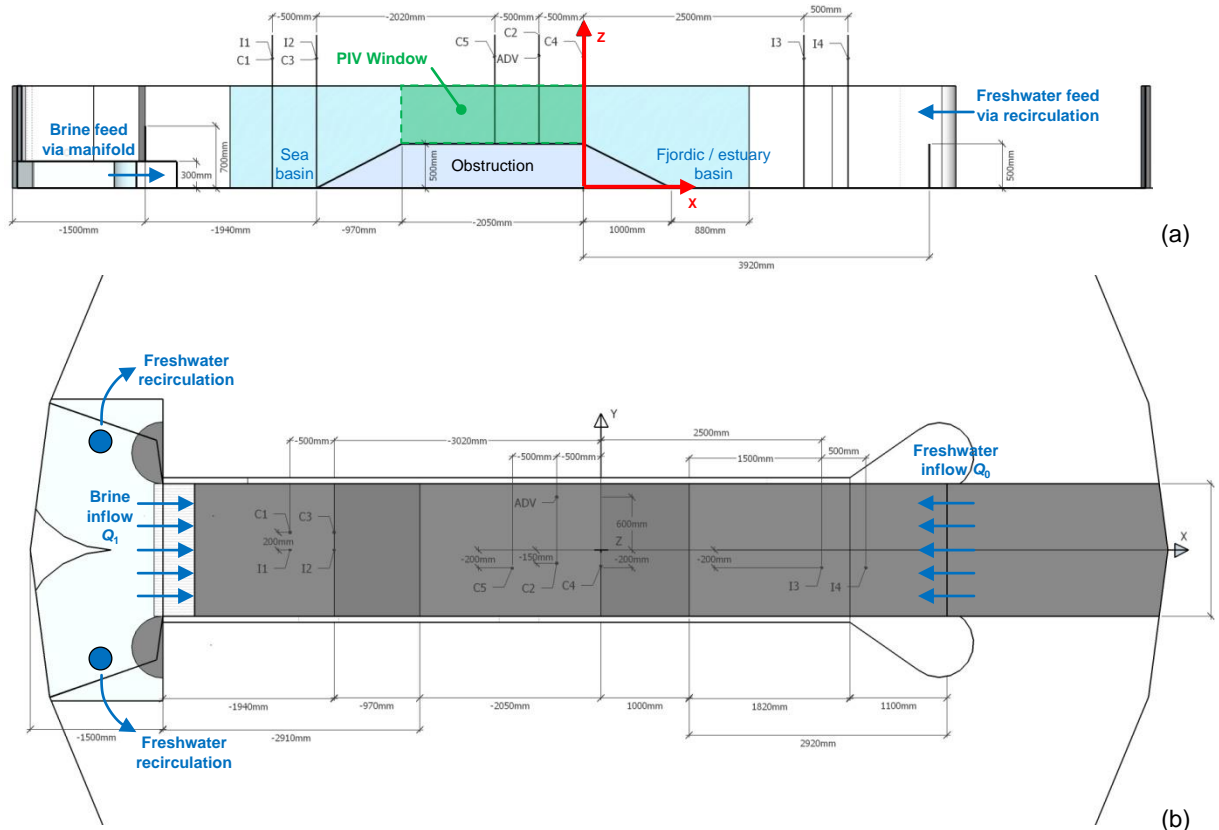
Figure 2. Schematic representation of the experimental set-up and instrumentation locations: (a) side view and (b) top view, showing directions of counter-flowing freshwater and brine inputs. Note: the figure orientation is opposite to that shown in Figure 1.
