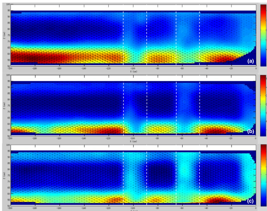
Figure 3. Time-averaged velocity fields across the sill obstruction [PIV window, Figure 2(a)] showing counter-flowing exchange flow generated in estuary run 4 ( h_s/H = 0.47 , \Delta\rho/\rho = 0.0096 ) under different Q_0/Q_1 inflow conditions of (a) 0 (i.e. Q_0 = 0 ); (b) 0.12; (c) 0.72.
