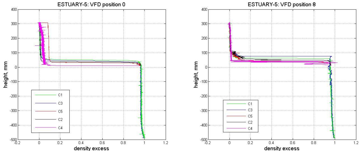
Figure 4. Measured density profiles C1 – C5 [probe positions shown in Figure 2(a) and (b)] generated in estuary run 5 ( h_0/H = 0.59 , \Delta\rho/\rho = 0.0096 ) under different Q_0/Q_1 inflow conditions of (a) 0 (i.e. Q_0 = 0 ) and (b) 0.44. Note that for profiles C2, C4 and C5, the crest elevation ( z' = 0 ) is the lower limit of these profiles.
